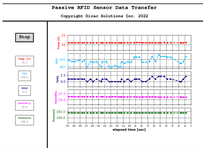
Figure 5. Graphical user interface showing time series data collected from multiple sensors inside the containment room reported by the inside small passive RFID tag through the containment wall.
