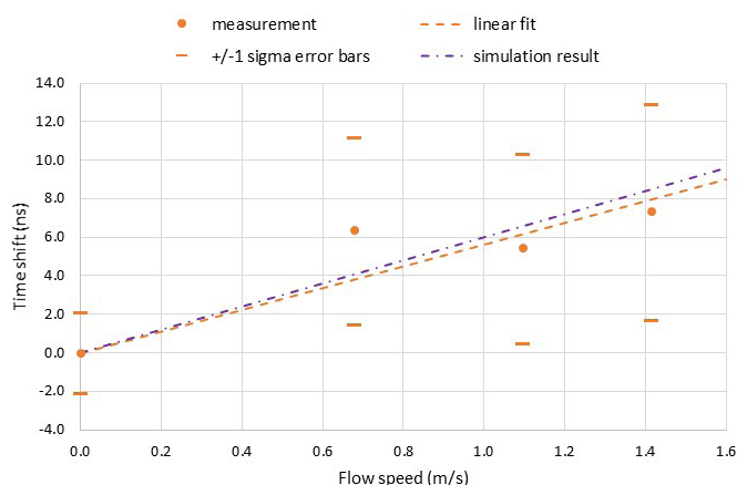
Figure 3. Correlation between LUS time difference signal and known flow speed.
