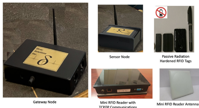
Figure 2: Components of WISLO system uses sensor network nodes and passive RFID through-wall communication transceivers.
