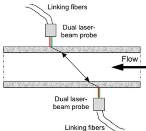
Figure 2. IOS concept for laser ultrasonic flow sensing, showing cross-section through a flow pipe.
