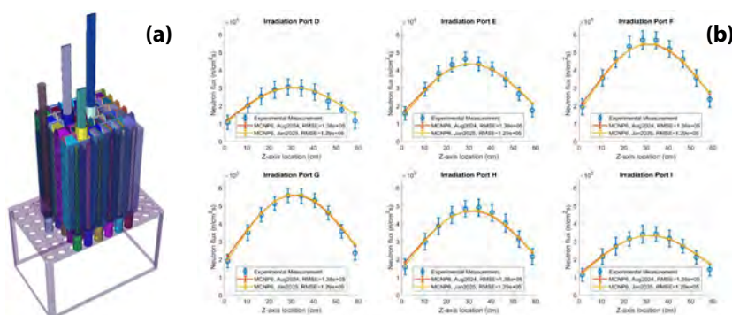
Figure 1. (a) Geometry and (b) Preliminary Experimental Validation of PUR-1 Neutronics Model
