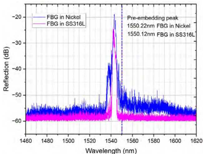
Figure 17. Reflection spectra of FBGs embedded in SS316L and nickel fabricated at 600°C measured at room temperature.
