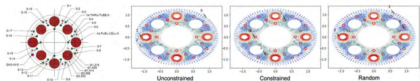
Figure 10. Graphite holder for the TRISO irradiation experiment.
