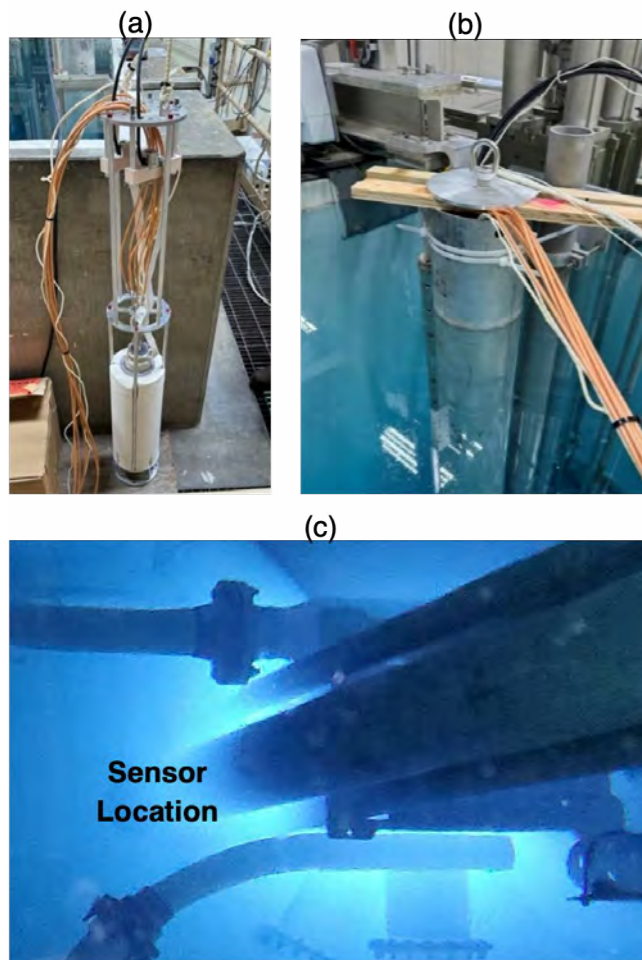
Fig. 25. (a) High temperature test rig loaded with a set of seven LGS SAWR sensor probes. (b) Vertical steel dry tube in the reactor pool, showing low temperature RF cables extending from the tube. The RF cables connect the sensor probes located in the furnace at the bottom of the dry tube to a DAQ system located on a nearby benchtop for in-situ sensor monitoring. (c) A view looking down into the reactor pool during high temperature / high irradiation LGS SAWR sensor testing. Reproduced from [3]
