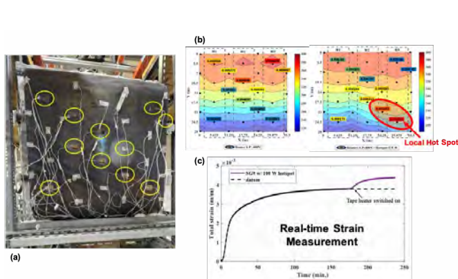
Figure 14. Laboratory Model of a Vessel Reactor Wall for Thermal-Mechanical Measurements (32 Thermocouples and 11 Strain Gauges) (a) Photograph of the Instrumented Vessel Wall; (b) Temperature and Strain Distributions for “Normal” and “Incident” Conditions; (c) Real-Time Strain Measurements Indicating when the Hot Spot was Detected by a Nearby Strain Gauge
