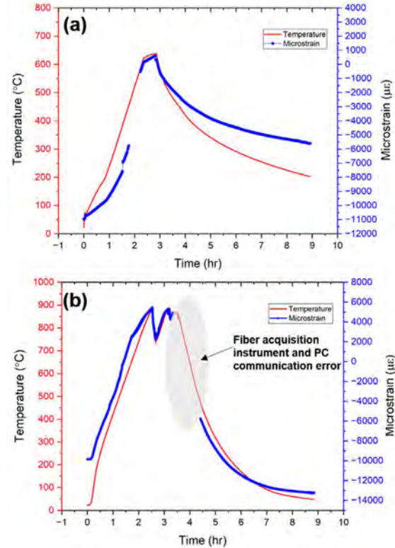
Figure 19. Evolution of FBG strain as a function of temperature up to (a) 700°C and (b) 900°C for the FBG embedded in SS316L.
