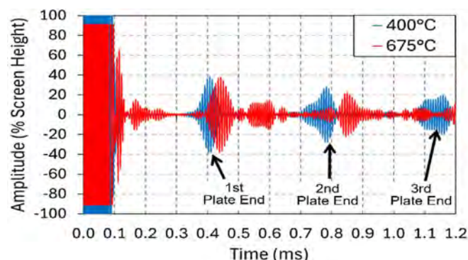
Figure 21. Electromagnet 400 and 675°C responses show clear plate end reflections. Responses at some temperatures were clearer than others.
