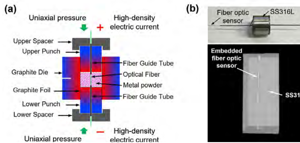
Figure 16. (a) Schematic representation of the embedding process using EFAS. (b) SS316L part with embedded fibers and X-ray computed tomography scan of the part
