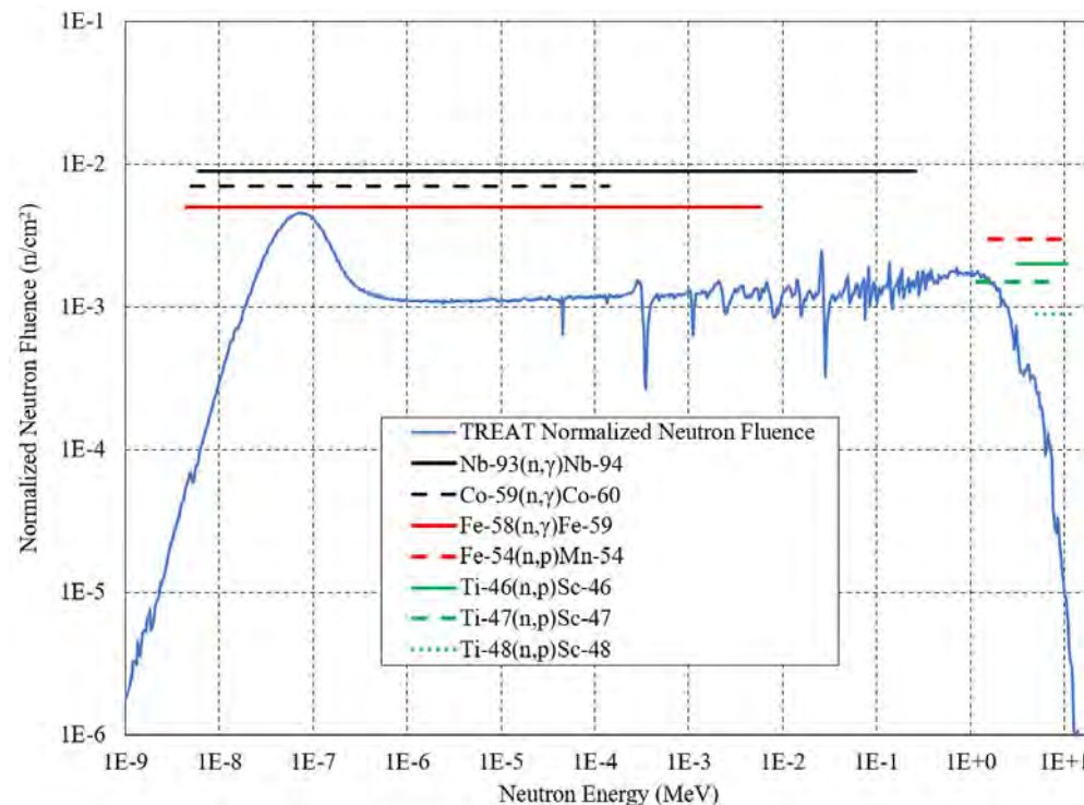
Figure 8. Normalized TREAT neutron fluence (blue) compared against energy coverage ranges for a selection of materials.
