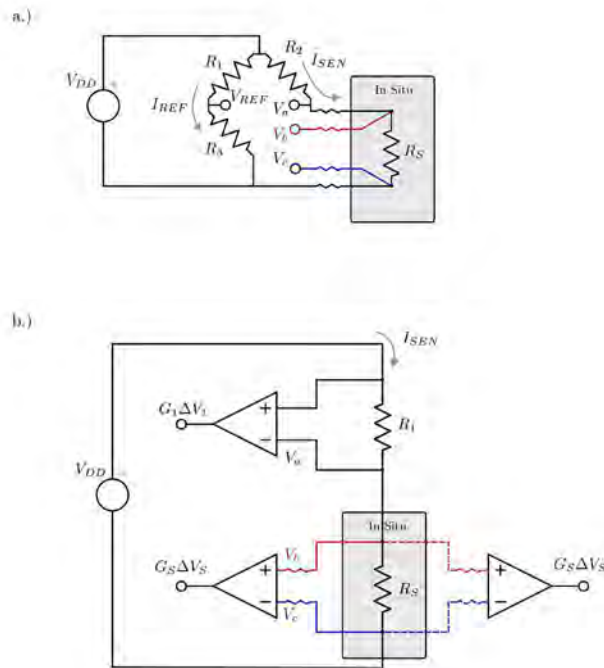
Figure 27. Resistance temperature devices (RTDs) can be performed in 2-, 3-, and 4-wire configurations using a bridge circuit (a.) or active components (b.)
