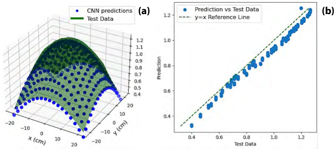
Figure 2. (a) Visualization of the CNN-predicted flux field (blue dots) overlaid on the test data (green surface) at 308 in-core locations. (b) Scatter plot comparing predicted and test values.
