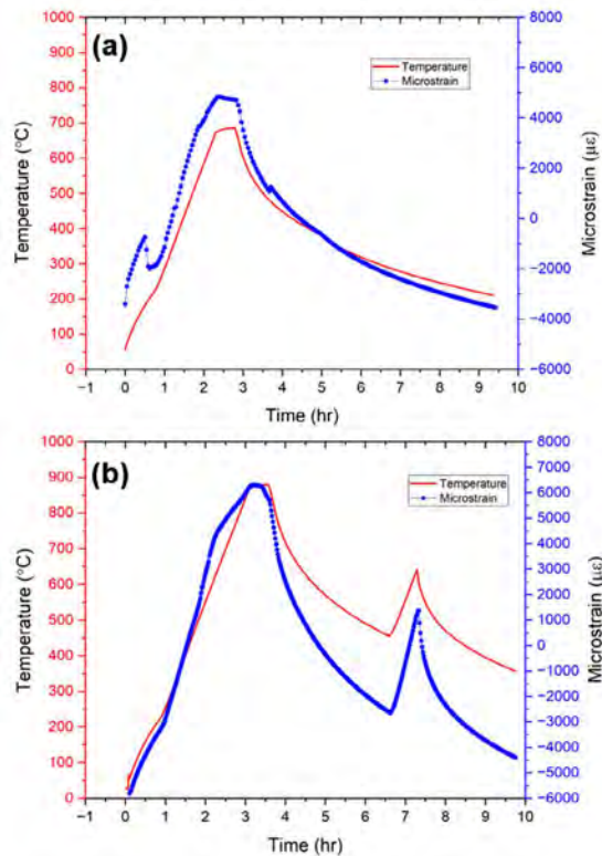
Figure 18. Evolution of FBG strain as a function of temperature up to (a) 700°C and (b) 900°C for the FBG embedded in nickel.
