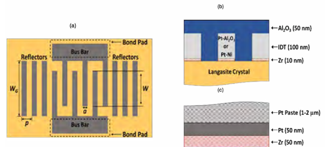
Fig. 23. (a) Top-view schematic of the SAWR sensor device. (b) Cross section of the device at the electrode region. (c) Cross section of the bond pad electrode on top of the bus bar region used for field coupling to the bus bars/interdigital transducer electrodes. Reproduced from [3].
