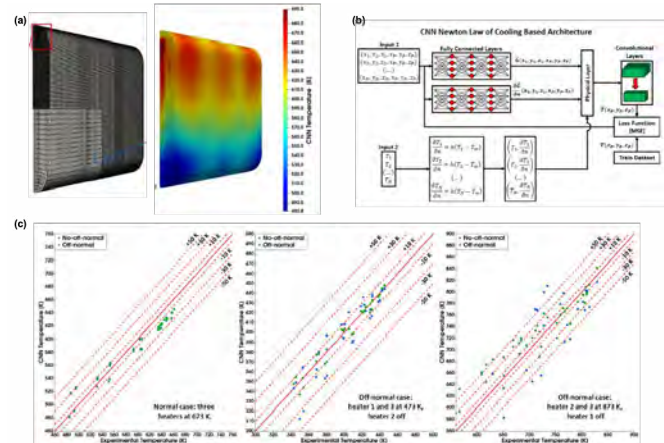
Figure 15. Reconstruction of the Vessel Temperature Field from the CNN (a) Sample Computational Model and Detailed Temperature Field Reconstruction; (b) CNN Architecture Coupling Radiative and Convective Heat Transfer; (c) Comparison of Local Temperatures Predicted by the CNN against Experimental Measurements for both Design and Off-Design Conditions
