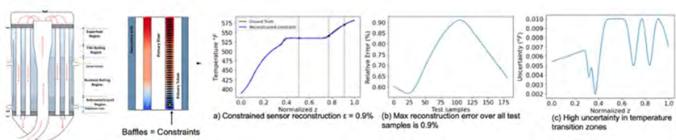
Figure 12. Steam generator design and temperature field reconstruction with the associated error and spatial uncertainty respectively.
