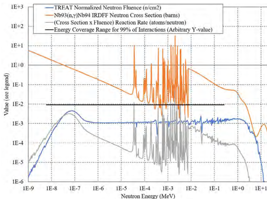
Figure 7. Normalized TREAT neutron fluence (blue) compared with ^{93}\text{Nb}(n,\gamma)^{94}\text{Nb} cross section (orange), reaction rate (gray), and energy range that incorporates 99% of interactions (black).
