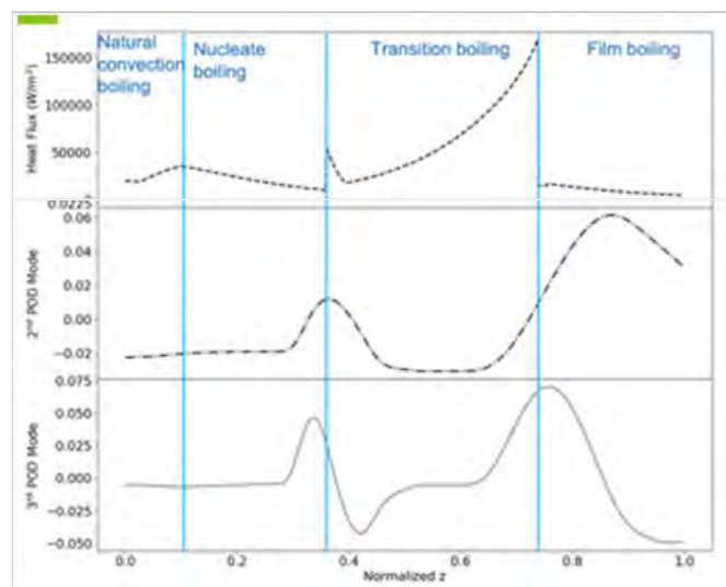
Figure 13. Reduced order model revealing interfaces between boiling mechanisms confirmed by the designer.
