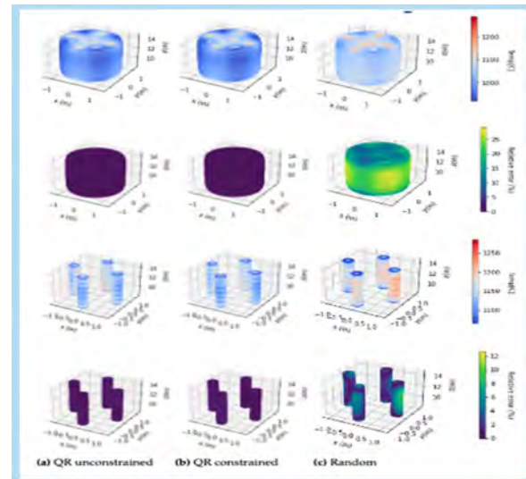
Figure 11. Holder field reconstruction, relative error, fuel temperature reconstruction, and relative error (Top to Bottom).
