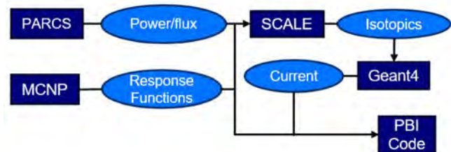
Figure 4. A flowchart which shows the data transfer between various codes to simulate power synthesis. Boxes indicate codes, while circles indicate data packets.
