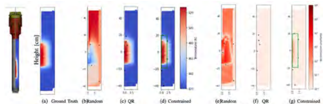
Figure 9. OPTI-TWIST temperature Reconstruction.
