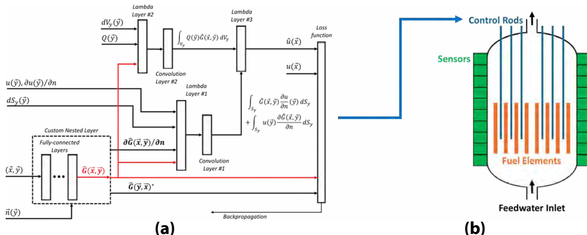
Figure 3. (a) Configuration of the proposed CNN during the training stage. (b) The trained Green's function will be used to optimize the control rod maneuvering during the testing stage.
