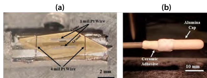
Fig. 24. (a) Top-view of a LGS SAWR sensor device attached and electronically connected to a high temperature Inconel cable. (b) The same device shown in (a) packaged/protected with an alumina cap using a high temperature ceramic adhesive. Reproduced from [3].
