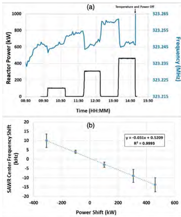
Fig. 26. (a) Representative LGS SAWR sensor with Pt-Al 2 O 3 electrodes showing frequency response at 800°C versus different reactor power levels. (b) Average frequency shift versus reactor power shift. Reproduced from reference 3.
