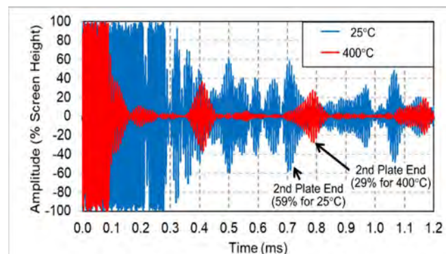
Figure 20. AlNiCo permanent magnet response at 25°C and 400°C showing the 2nd plate end reflection at 400°C to be 29% of 25°C response.
